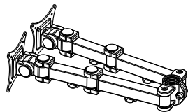
(2) VESA Plate with Arm Assembled-c
